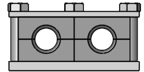
2 HOLE CLAMP 50630
