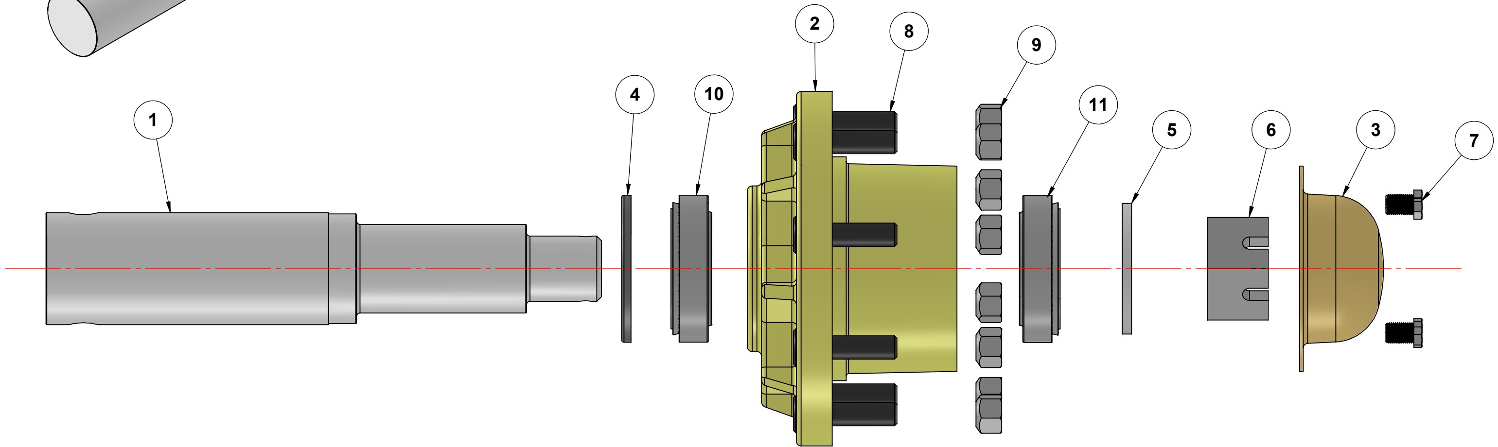
HUB ASSEMBLY
