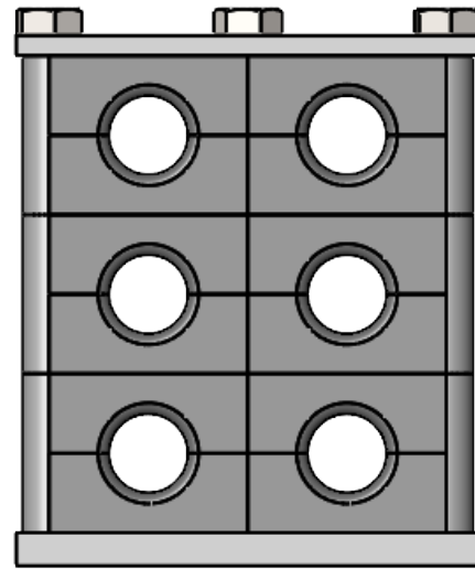
6 HOLE CLAMP 50627
