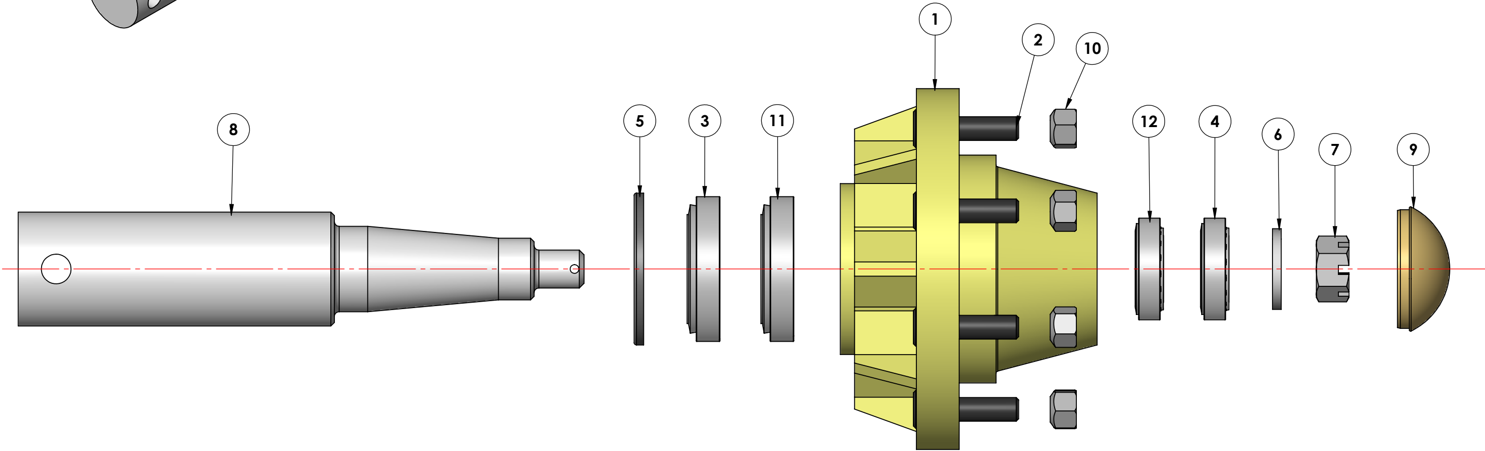
HUB ASSEMBLY
