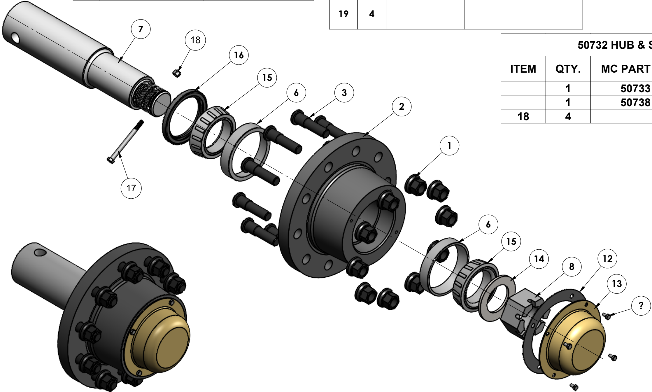
50732 HUB ASSEMBLY
