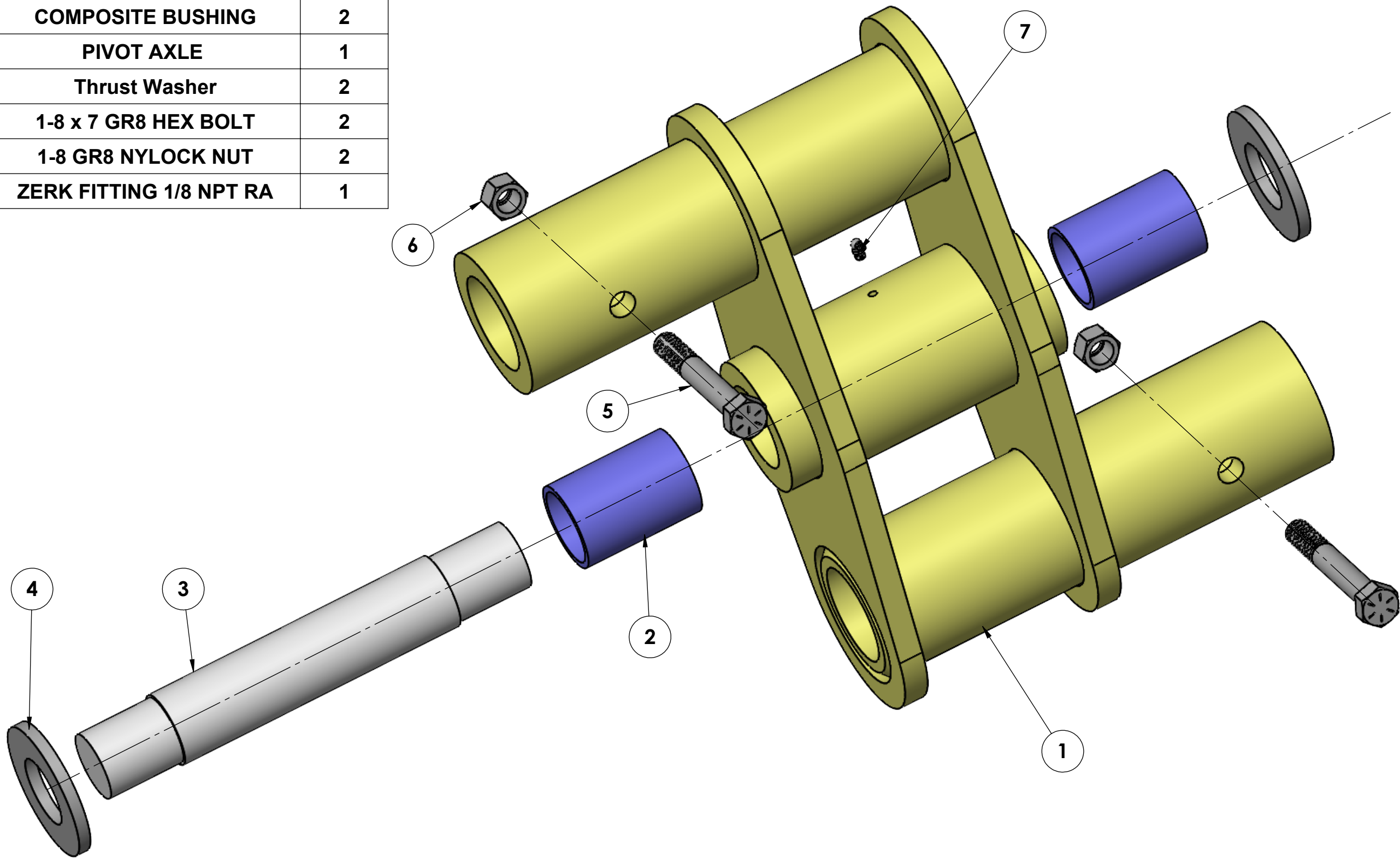
OSCILLATOR ASSEMBLY
