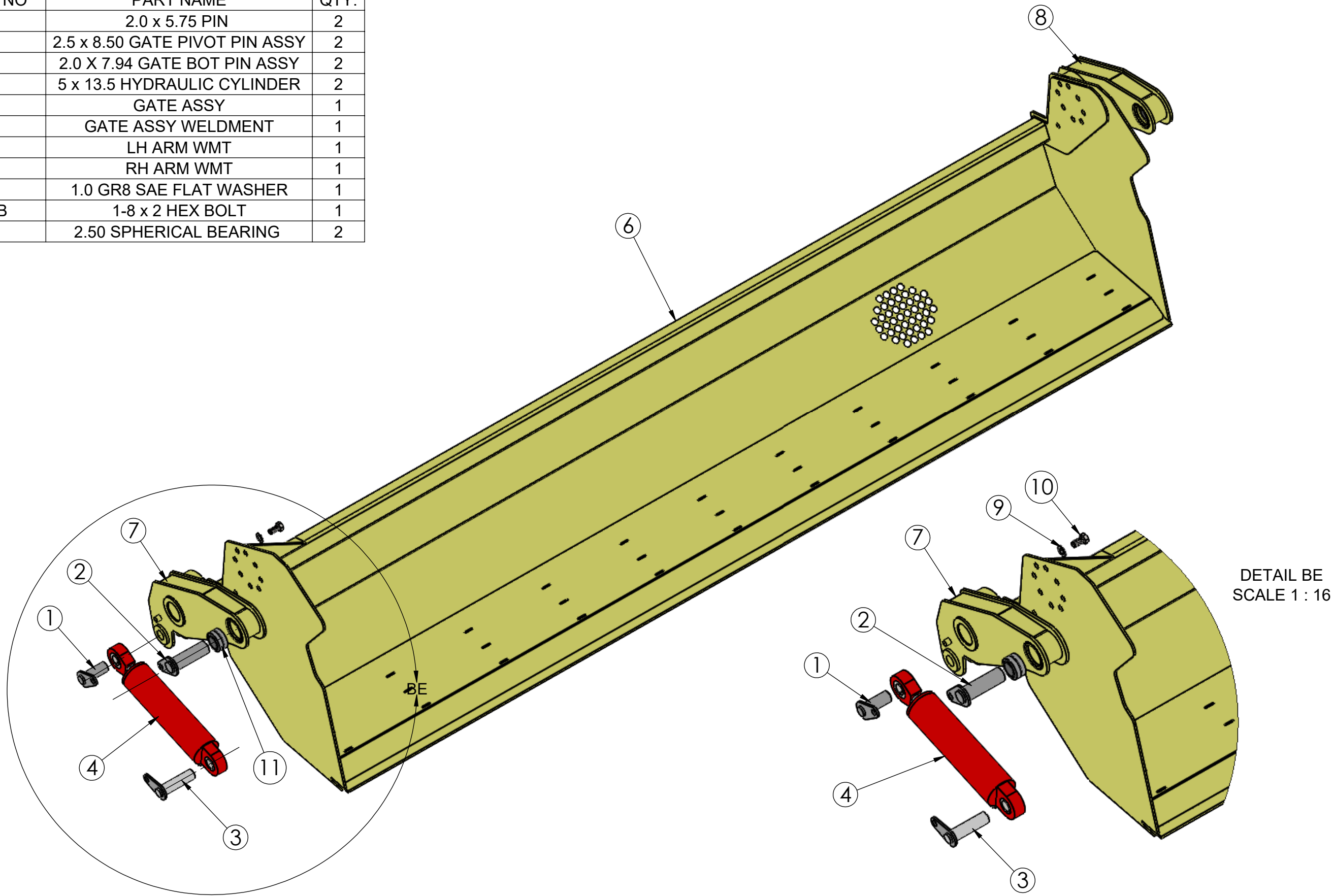
36305 GATE ASSEMBLY
