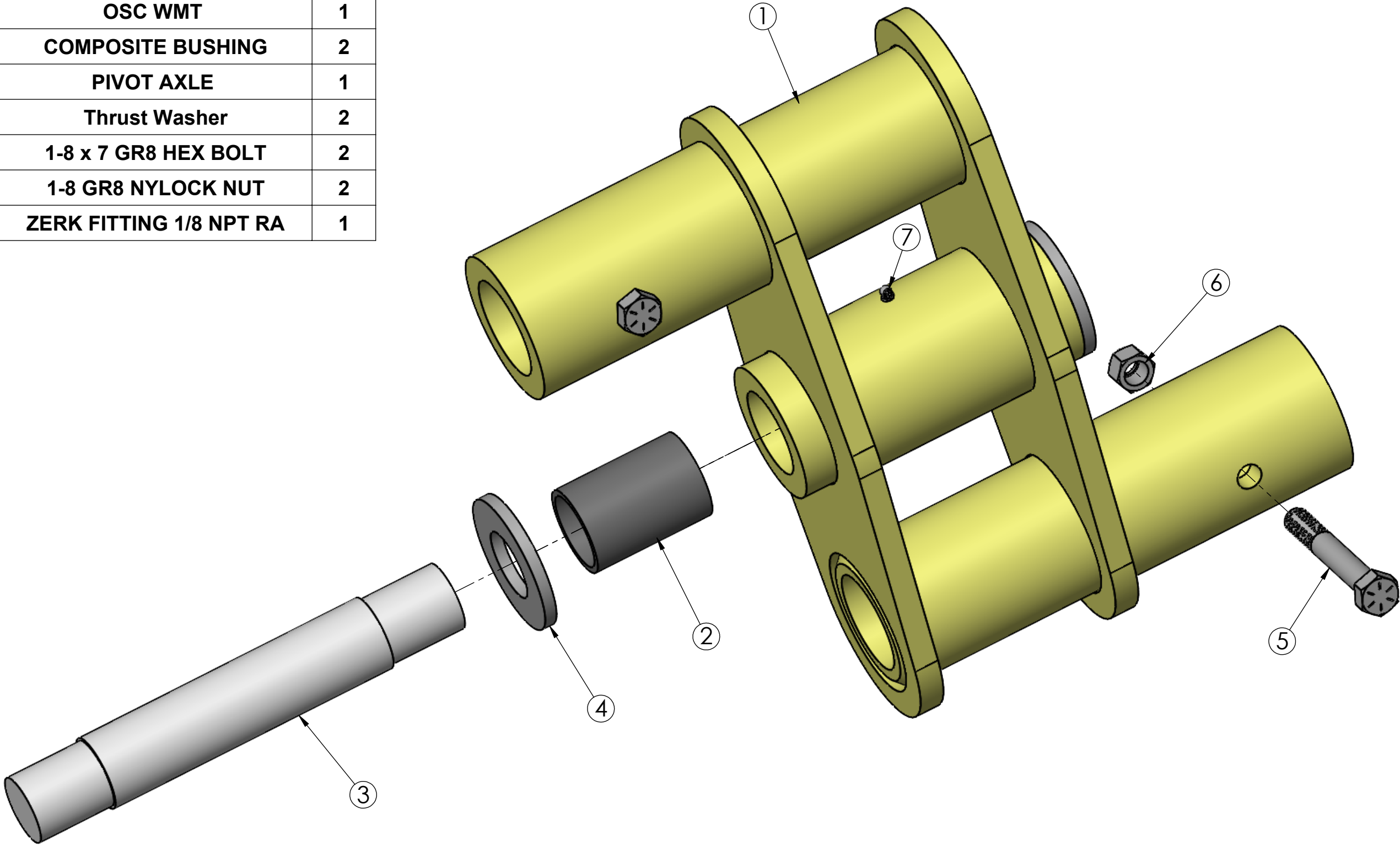
OSCILLATOR ASSY
