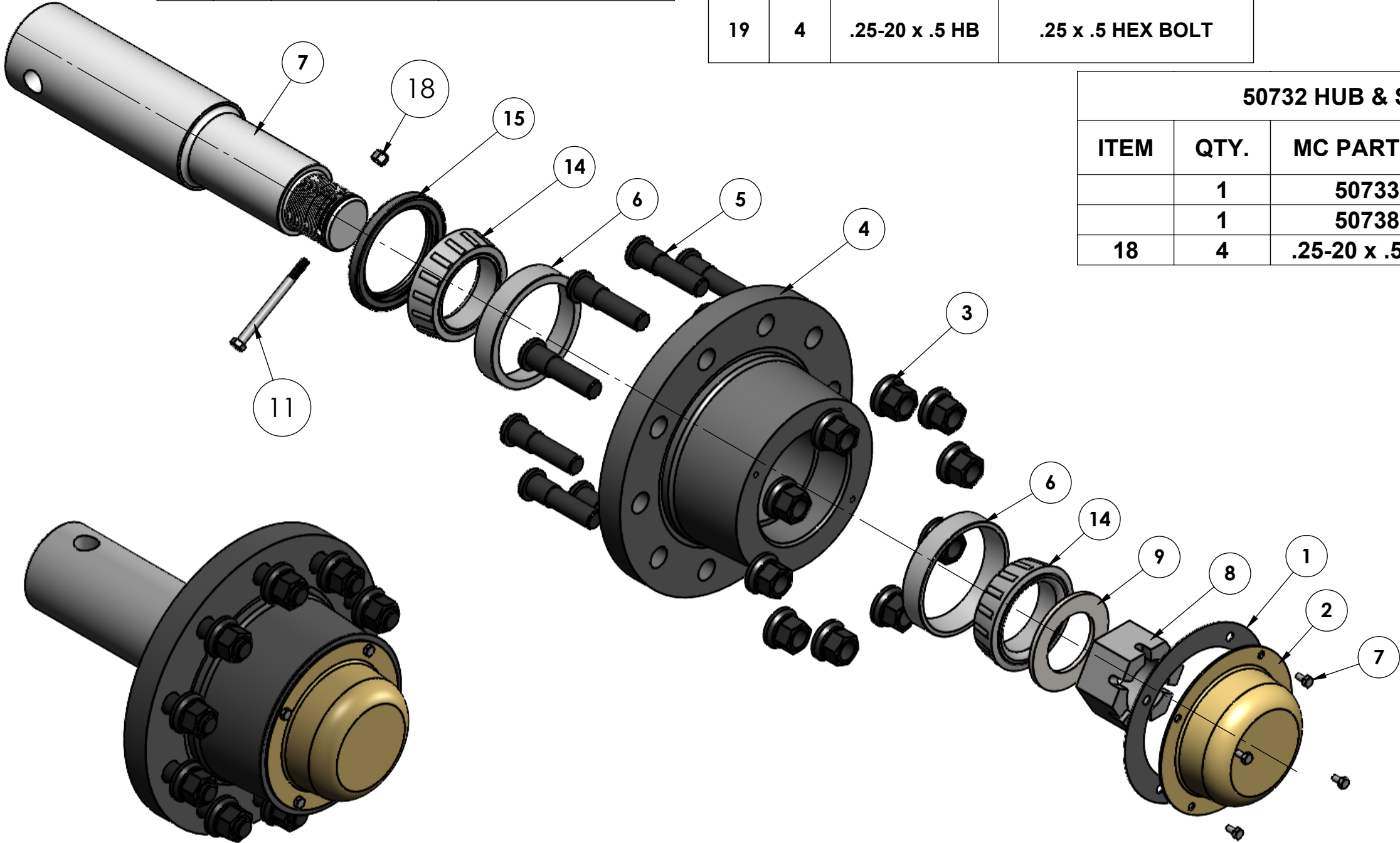
50732 HUB ASSEMBLY
